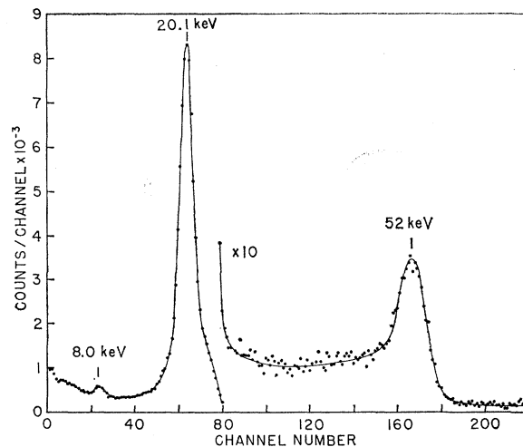
FIG. 3. Singles gamma-ray spectrum of Rh 104m obtained with a proportional counter.
