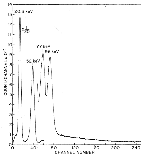
FIG. 2. Singles gamma-ray spectrum of the 4.4-min isomer of \text{Rh}^{104m} obtained with a 1\frac{1}{2} in. \times 1 in. NaI(Tl) scintillation spectrometer.
