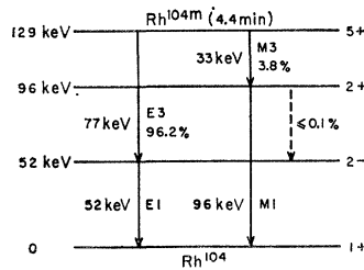
FIG. 8. The isomeric gamma-decay scheme of \text{Rh}^{104m} .
