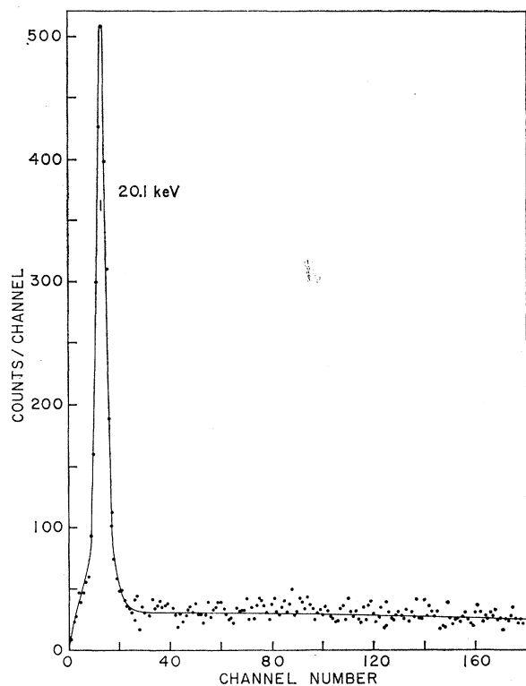
FIG. 6. The Rh 104m gamma-ray spectrum in coincidence with 96-keV gamma rays.
