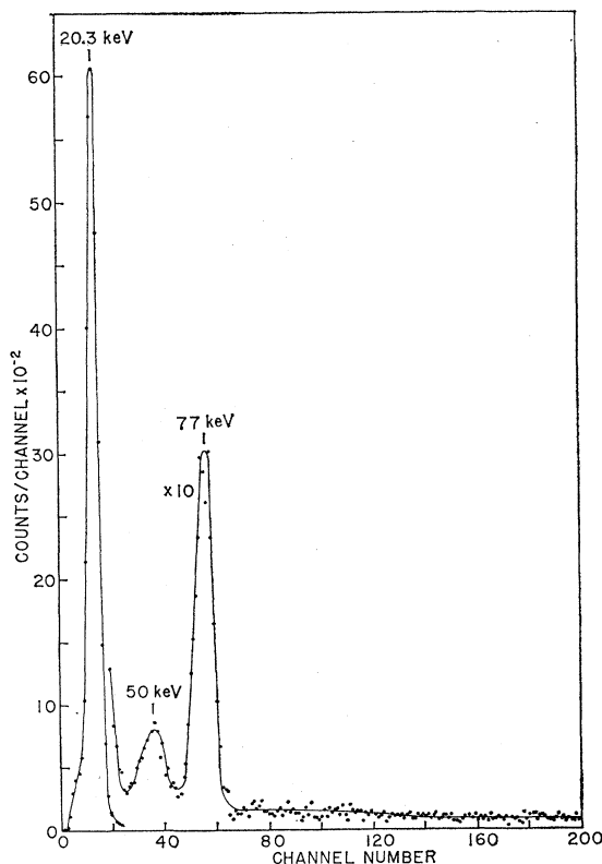
FIG. 5. The \text{Rh}^{104m} gamma-ray spectrum in coincidence with 52-keV gamma rays.
