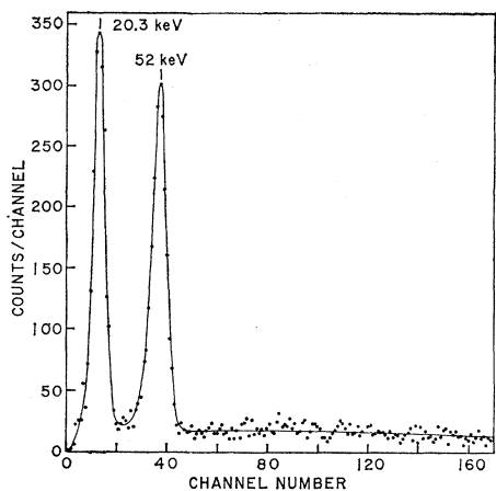
FIG. 4. The \text{Rh}^{104m} gamma-ray spectrum in coincidence with 77-keV gamma rays.
