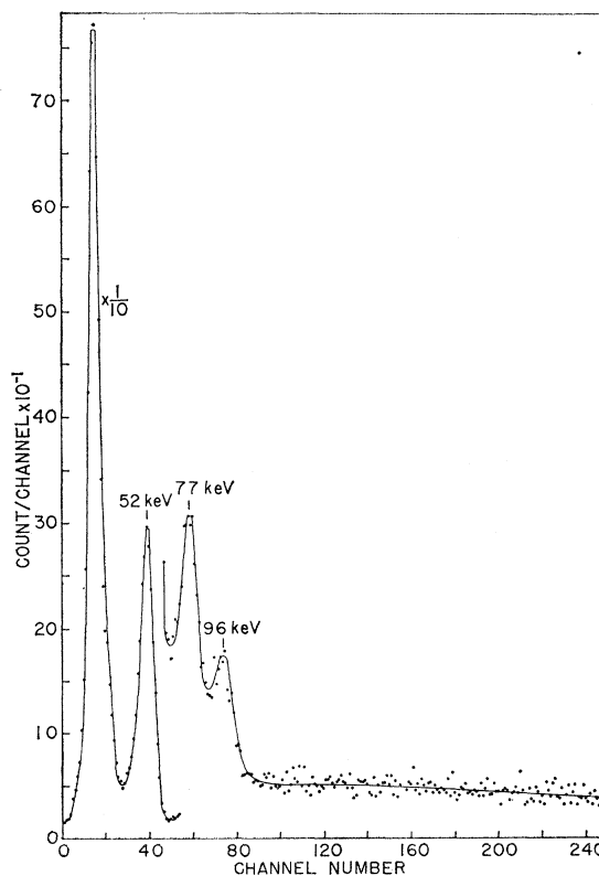
FIG. 7. The Rh 104m gamma-ray spectrum in coincidence with rhodium K x rays.
