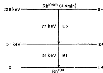
FIG. 1. The \text{Rh}^{104m} decay scheme proposed by Jordan, Cork, and Burson (reference 10).
